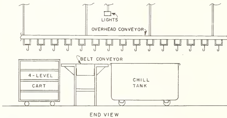
Figure 10.--Layout of turkey grading area in plant E.
